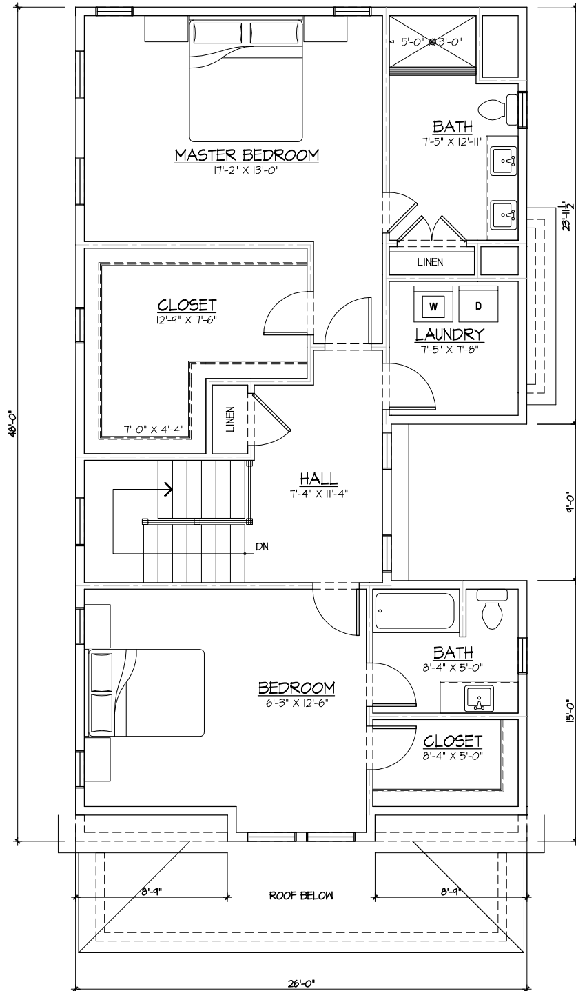
Second Floor [1,151 SF]
