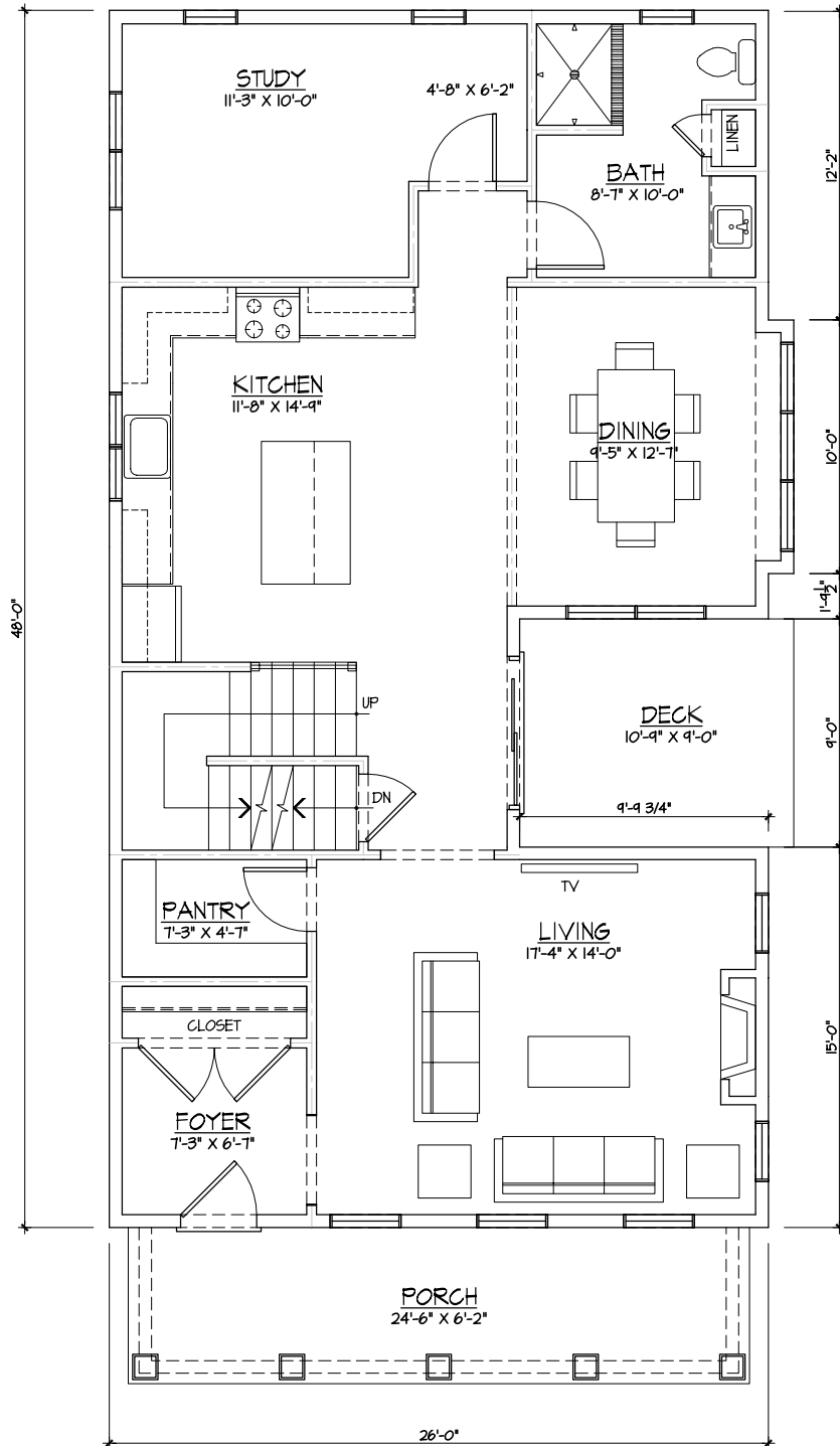
First Floor [1,170 SF]
